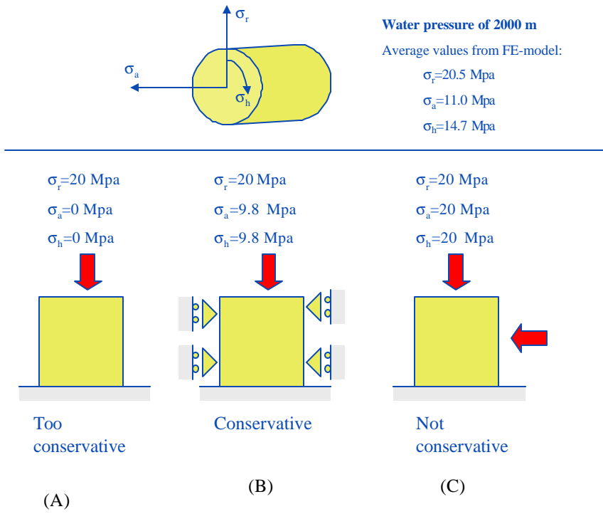
Figure 3. Stress Analysis for Submerged Insulated Flowline and Three Corresponding Test Methods
