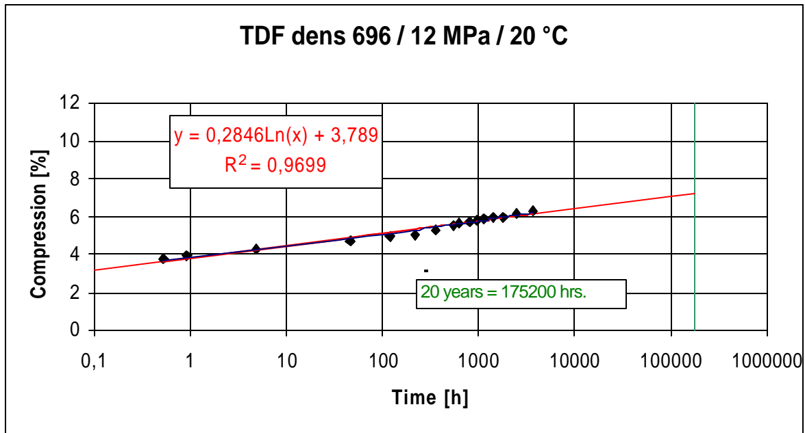
Figure 6. Creep Curve, 3712 hours for Novel PP foam
