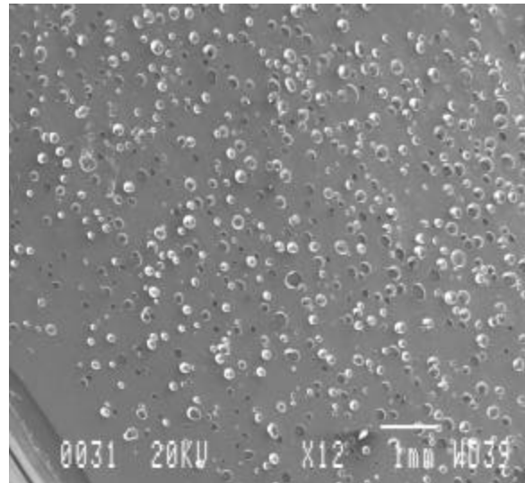
Figure 2b. SEM Photograph Novel PP Foam
