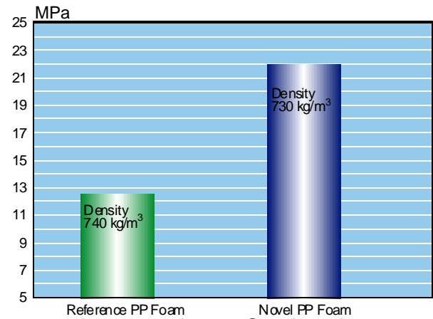
Figure 5. Compressive Strength @ 5% Strain Comparison
