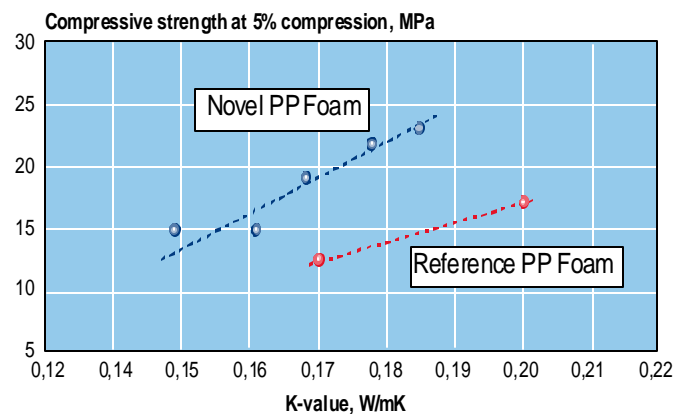
Figure 7. Thermal Conductivity vs. Compressive Strength
