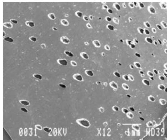
Figure 2a. SEM Photograph Reference PP Foam
