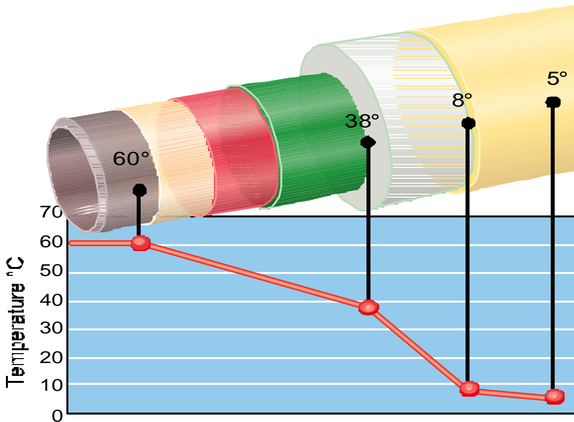
Figure 8. Temperature Profile Through layers for a Deep Water Design
